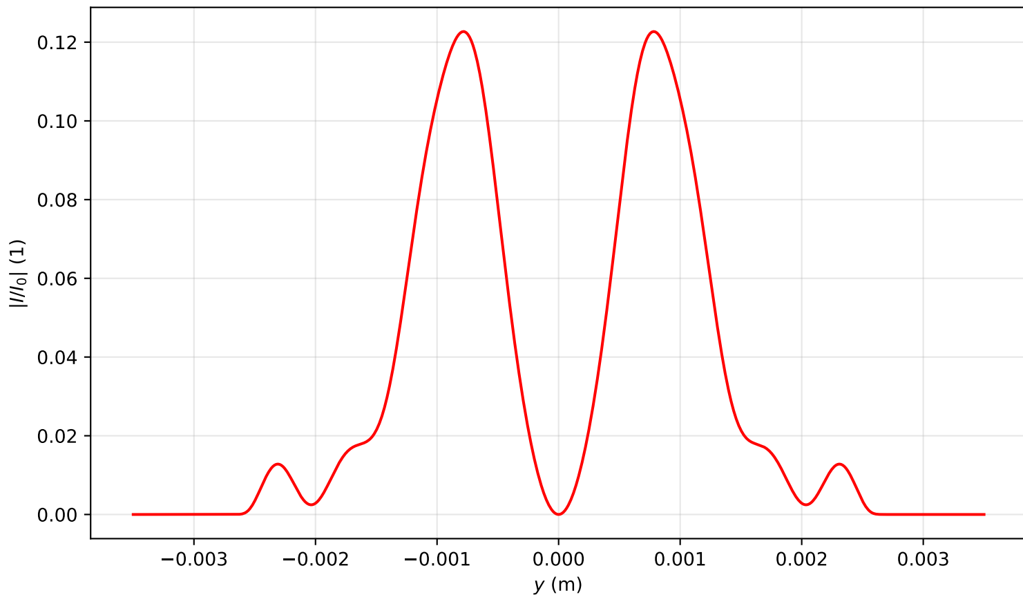
Intensity profile I(x=0, y, z=3.423)/I_0 , \text{Pin}=4.0\text{Pcr} , artificial time
